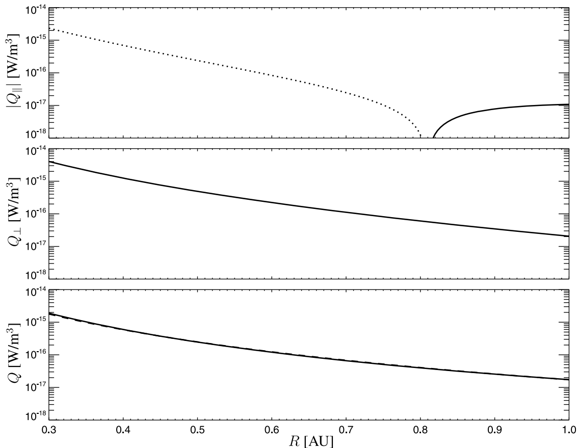
Figure 7. Estimated heating rates from the fitted data (assuming a decelerating solar wind, equation (11)): (top) absolute value of the parallel heating rate Q_{\parallel} (Dotted line denotes negative values of Q_{\parallel} , whereas solid line denotes positive values.), (middle) perpendicular heating rate Q_{\perp} , and (bottom) average heating rate Q . The dashed line displays the fitted result, equation (12).
