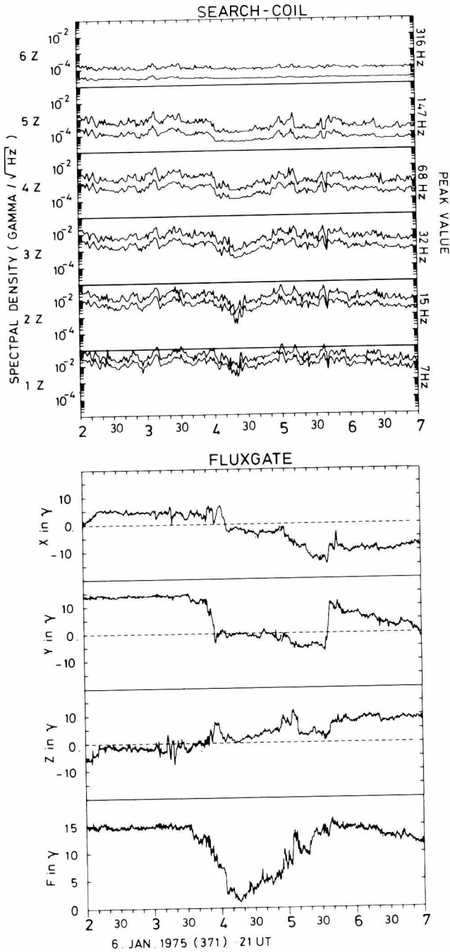
Fig. 6. "Magnetic hole" with pronounced dip in magnetic wave activity
