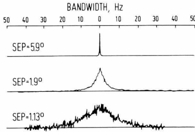
Fig. 3. Spectral distribution of the amplitude of received S-band radio signal ( 1.13^\circ \approx 4.2 R_\odot )
