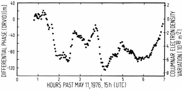
Fig. 7. Helios B electron content data closest to sun (west limb): May 11, 1976 (SEP = 1.55^\circ /p = 5.8 R_\odot )
