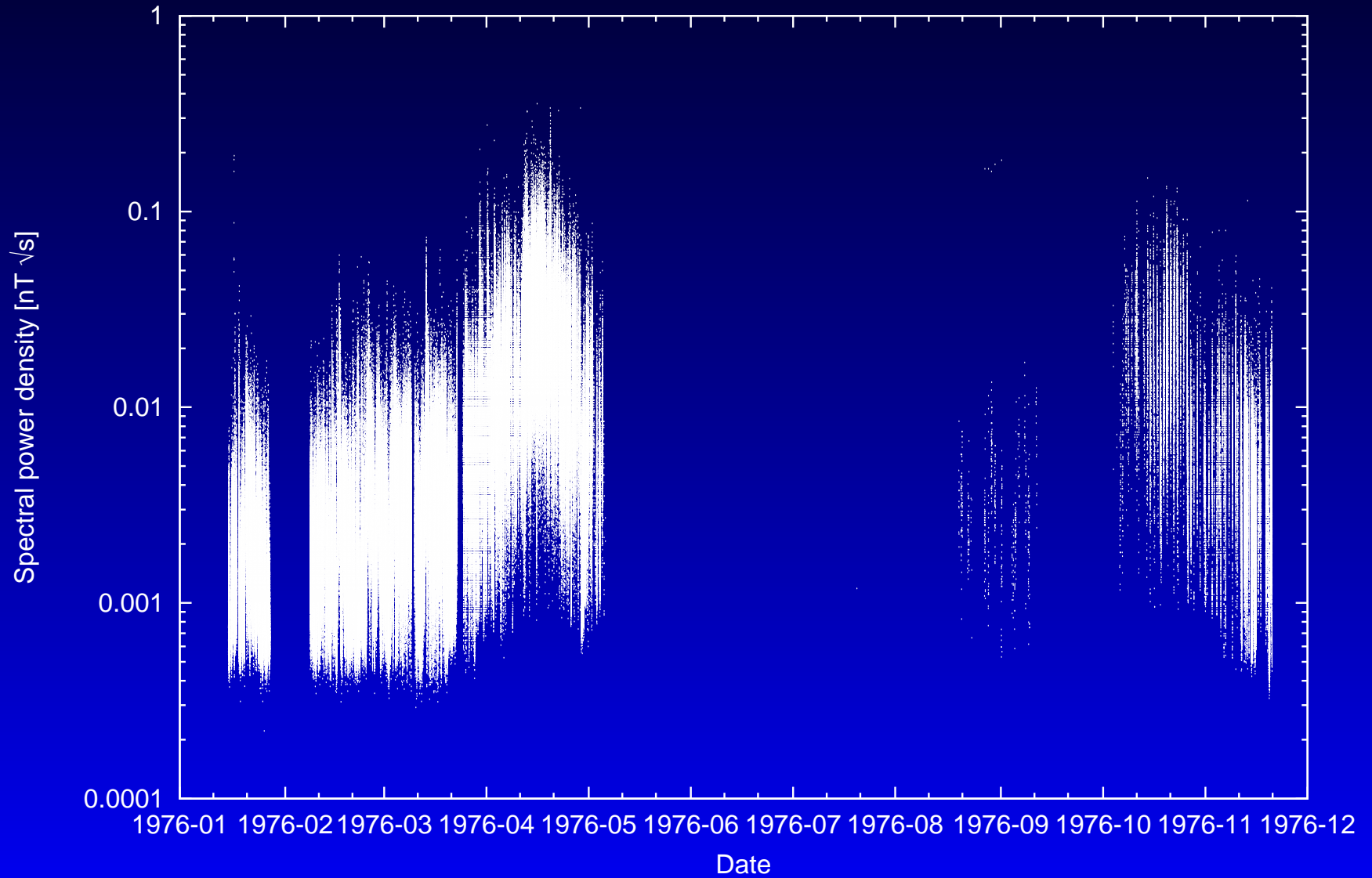
Helios 2 E4 sensor Z channel 1
