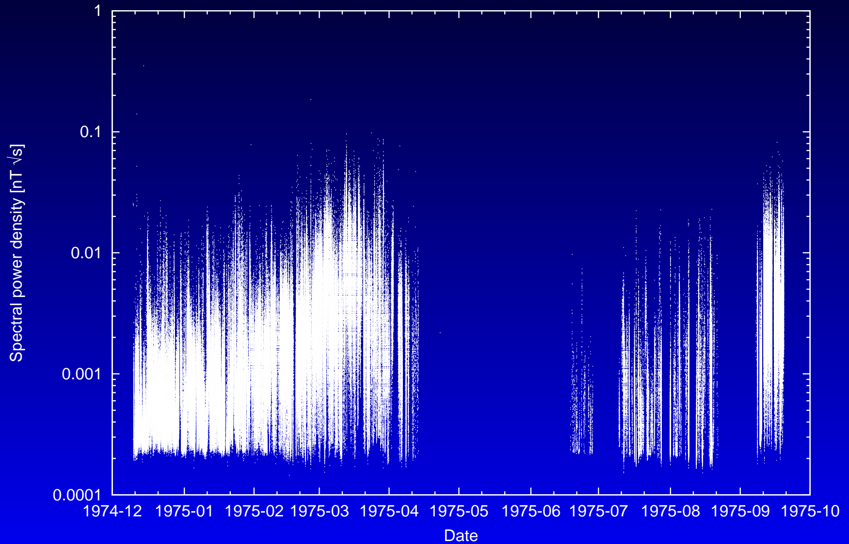
Helios 1 E4 sensor Z channel 2
